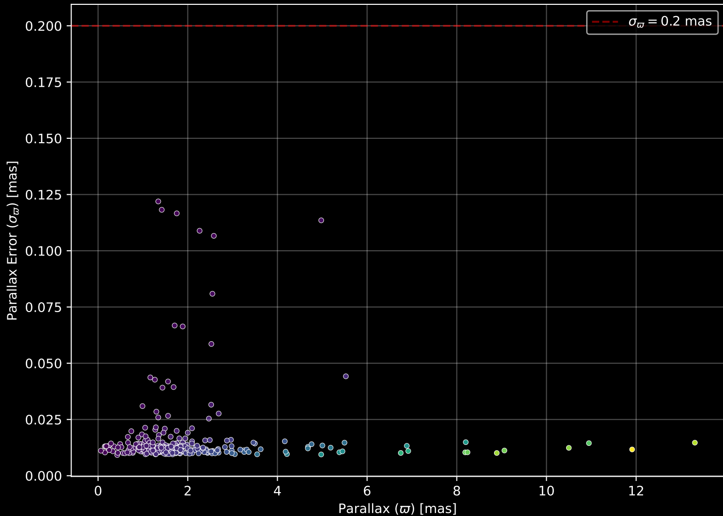
GALAH DR4 Field: [7010] Parallax Quality (n= 300)
