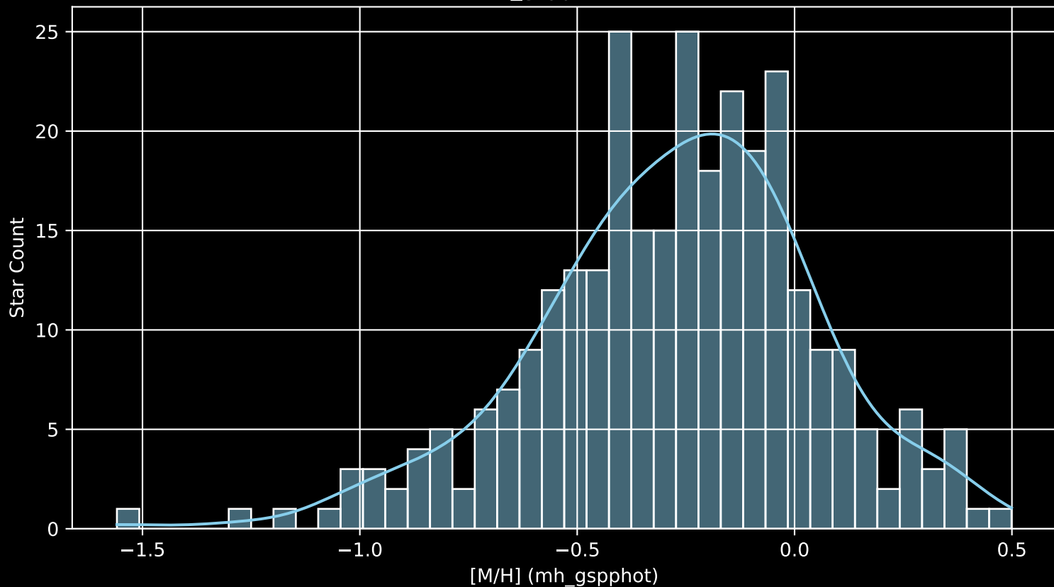
GALAH DR4 Field: [7010] [M/H] (mh_gspphot) (n= 298)
