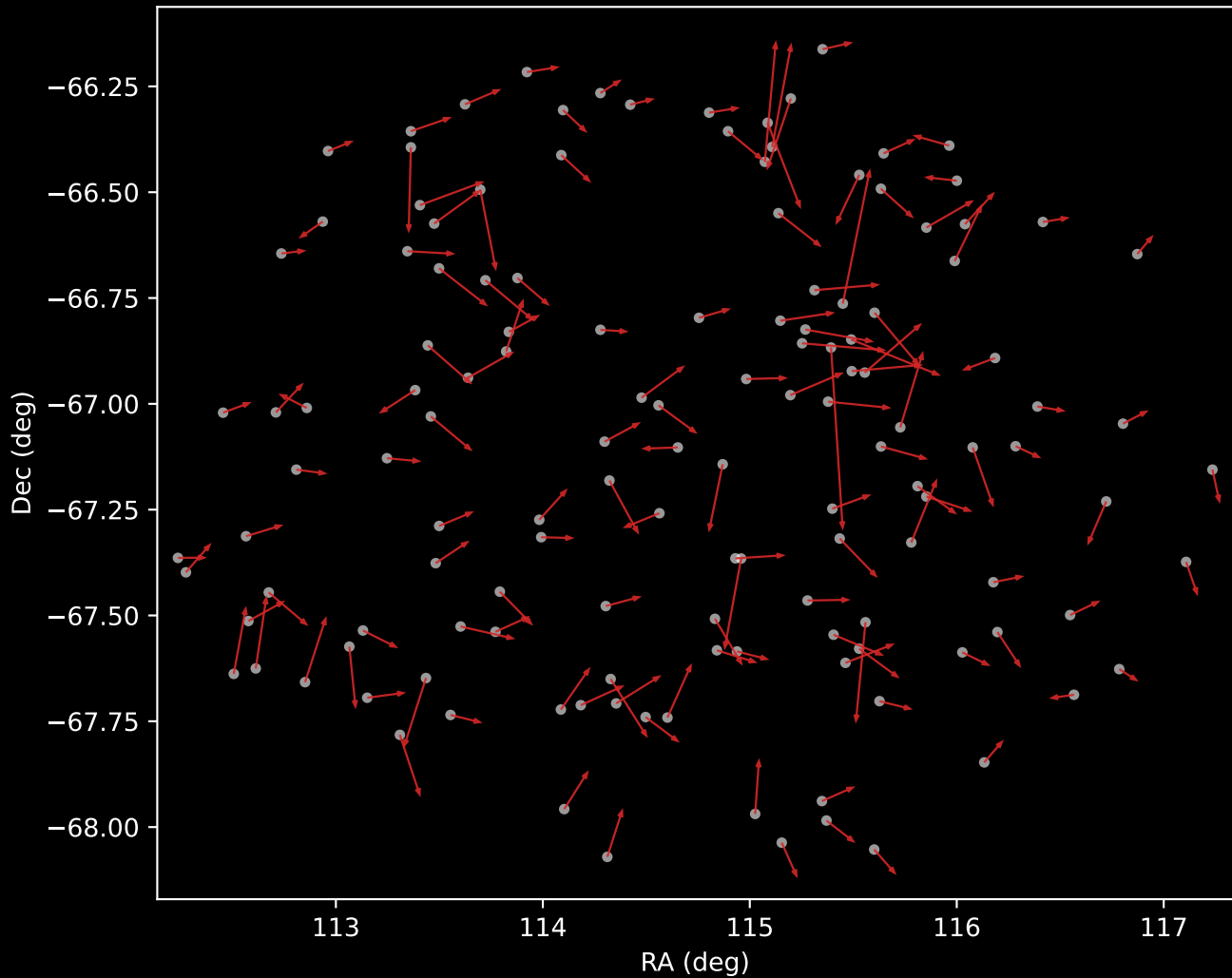
GALAH DR4 Cluster 6 Proper Motion Vectors (n=137)
