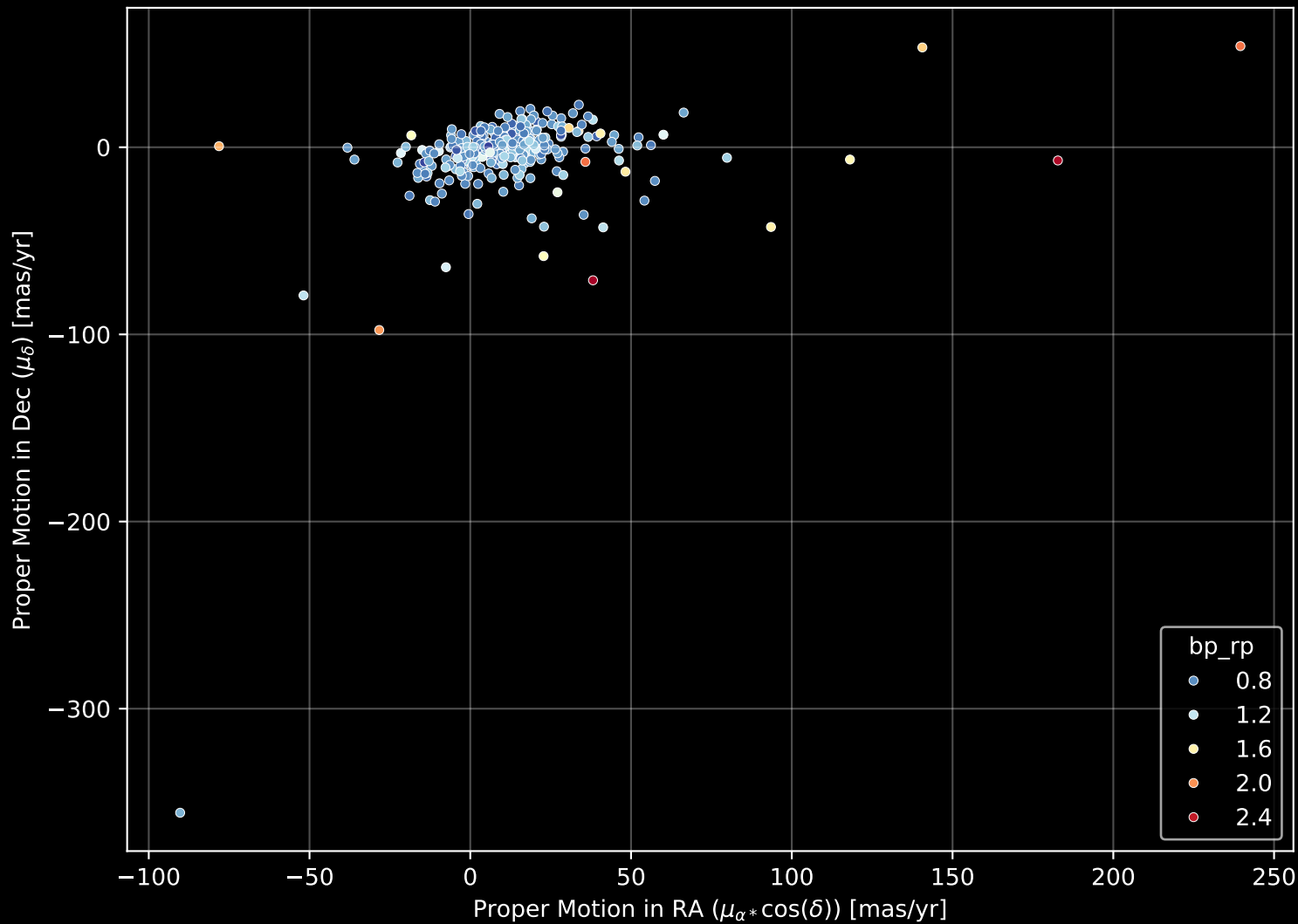
GALAH DR4 Field: [7010] Proper Motion Diagram (n= 300)
