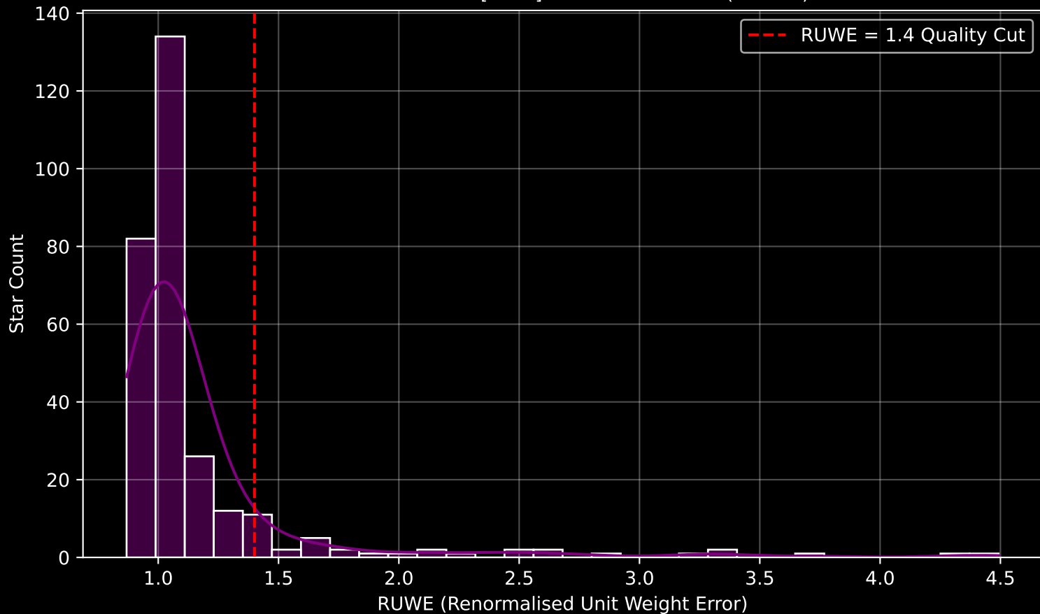
GALAH DR4 Field [7010] RUWE Distribution (n= 290)
