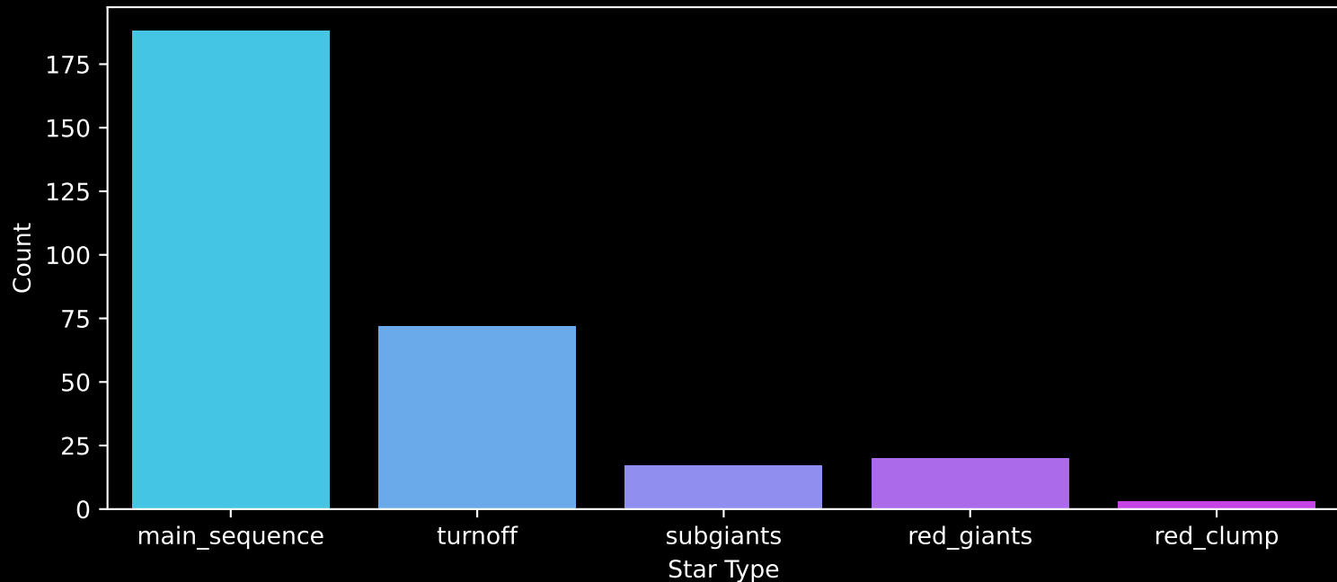
GALAH DR4 Field: [7010] Count plot of Star Type
